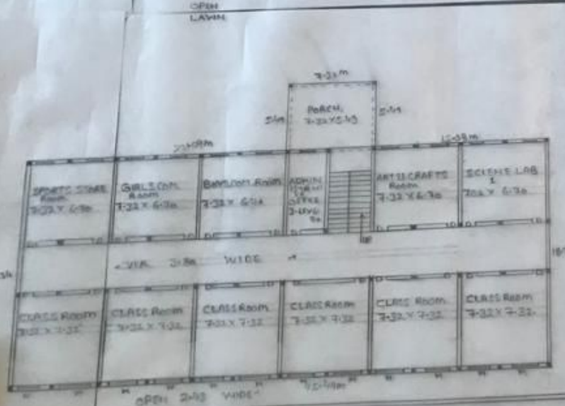
Exo Ground Floor Plan
